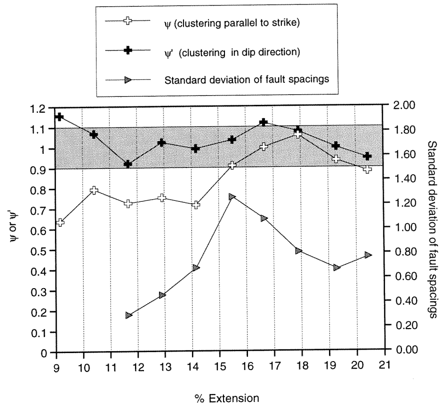
Figure 4.21: Scanline-based clustering dimensions and standard deviation of fault spacings through time. Shaded box represents a range of clustering dimensions interpreted as "random" (uniform) spatial distributions. Note the shift in the standard deviation trend is coincident with \psi entering the shaded region. See text for complete discussion.
