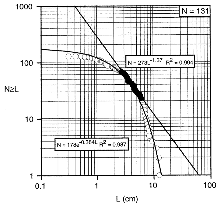
Figure 2.12: Cumulative frequency diagram of mode I fracture lengths for the bedding surface shown in Figure 11. It is not clear if there is a "flat" central segment suggestive of a power-law distribution of sizes. The data as a whole are better fit using an exponential function. If the data do indeed follow a power-law distribution, then truncation and censoring effects are severe for this sample (see discussion of Figure 2.15).
