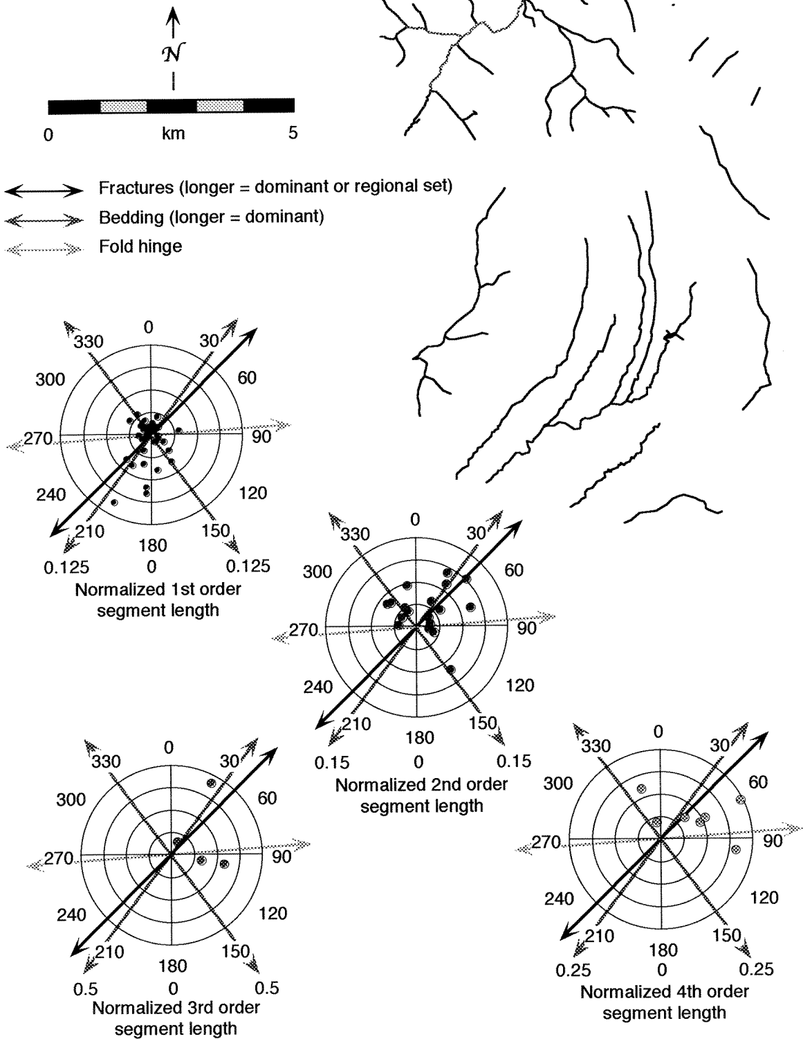
Figure 1.5: Streams, flow vector and structural data for Domain 7. See text for discussion.
