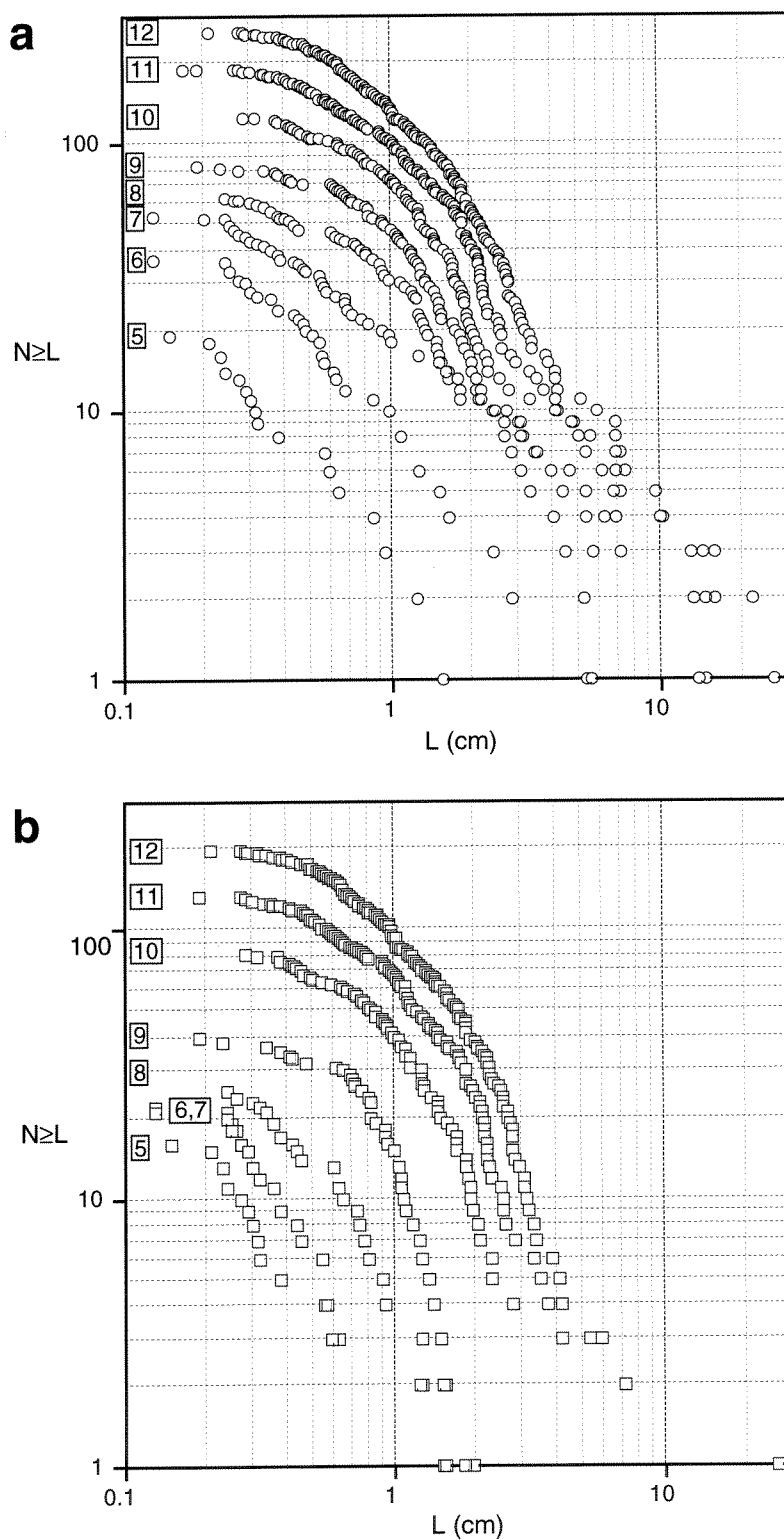
Figure 4.23: Cumulative frequency analysis of fault lengths for time steps 5 - 12 before (a) and after (b) faults believed to be related to edge effects are parsed from the data. Parsing appears to generally degrade the plots, although the degradation decreases with time. The change from a power-law to exponential distribution of fault sizes is still apparent.
