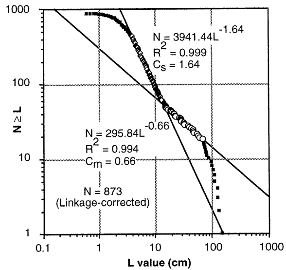
Figure 3.2. Cumulative frequency plot of fault lengths for all structures within a \sim 34 \text{ m}^2 area. Note the two distinct central segments, suggesting two subsets of faults, with slopes that differ by \sim 1.0 . Subscripts of m and s are for master faults and small faults, respectively.
