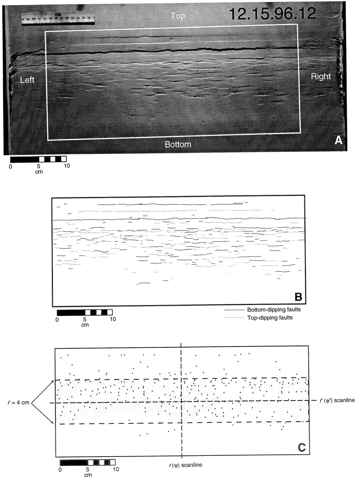
Figure 4.9: Time 12. A is the image of the model surface; the study area is outlined with the white box. B is the fault map derived from the image in A, C is the centroid map derived from B.
