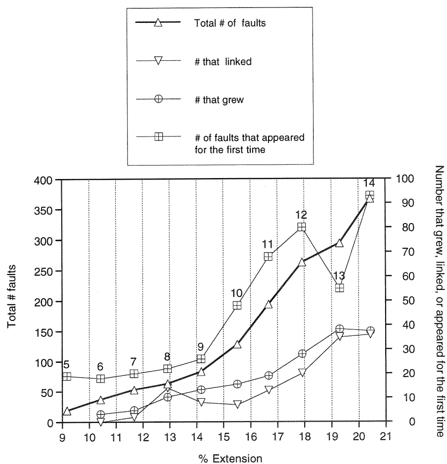
Figure 4.13: Absolute numbers of faults through time, unnormalized. Note that all numbers are increasing.
