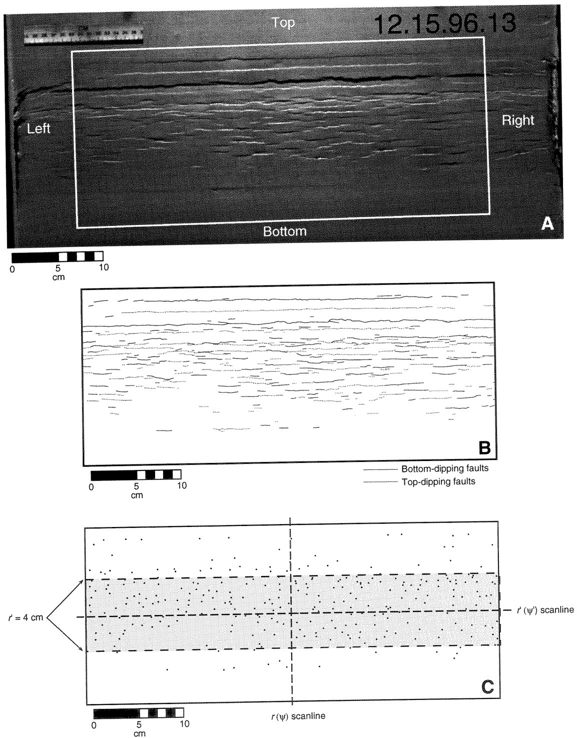
Figure 4.10: Time 13. A is the image of the model surface; the study area is outlined with the white box. B is the fault map derived from the image in A, C is the centroid map derived from B.
