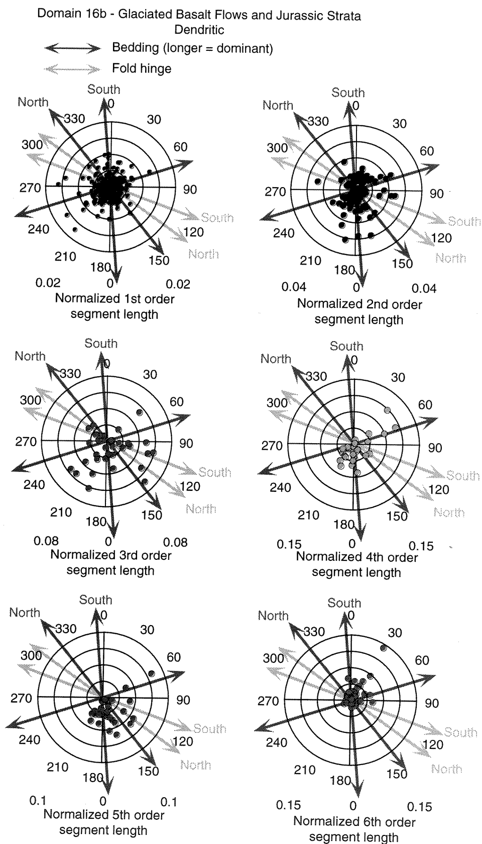
Figure 1.9b: Streams, flow vector and structural data for Domain 16b. See text for discussion.
