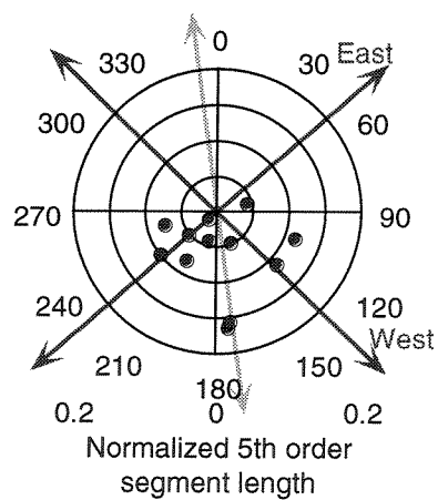
Figure 1.8b: Flow vector and structural data for Domain 16a. See text for discussion.
