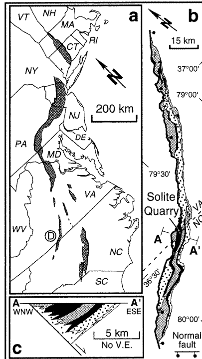
Figure 2.1: (a) Exposed Mesozoic rift basins of the eastern United States. D is the Danville basin. (b) Simplified geologic map of Danville basin, showing location of Solite Quarry. Black represents Cow Branch members of the Leekesville Formation. (c) Simplified geologic cross section of the Danville basin (see b for location), illustrating half-graben geometry modified by inversion. Modified from Olsen and Kent (1997), Schlische et al. (1996), and Schlische (1997).
