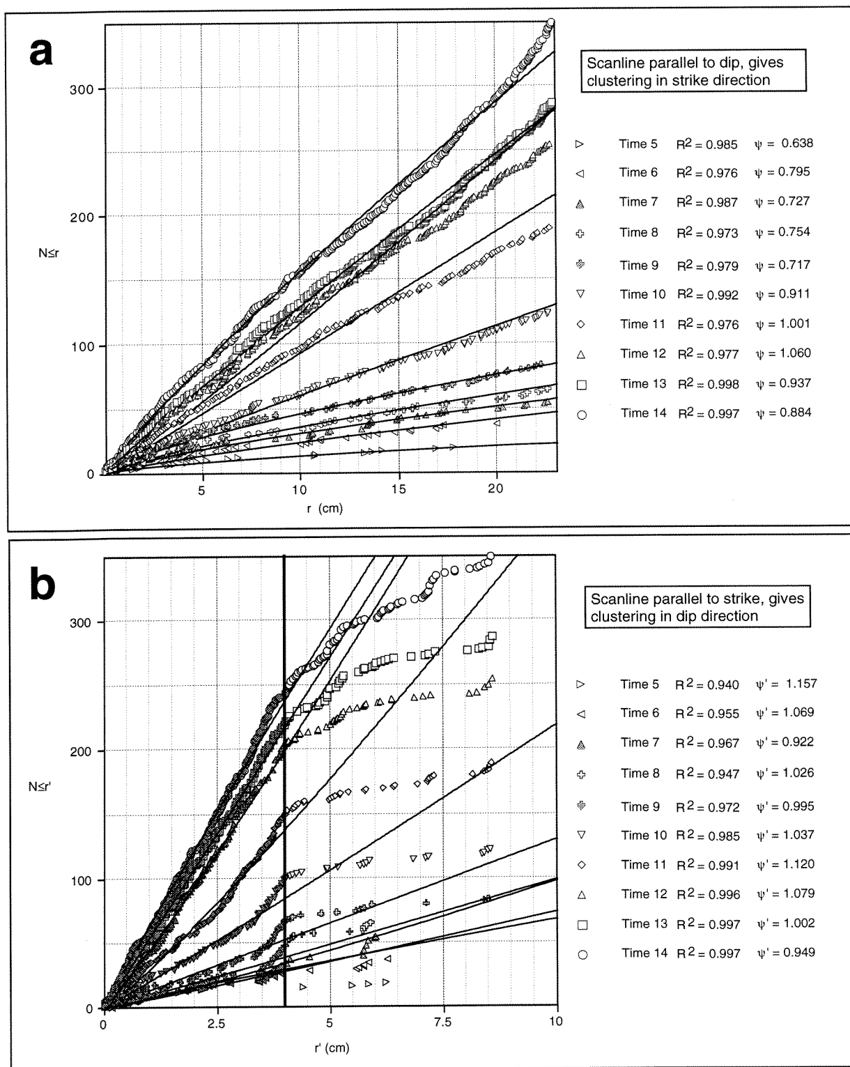
Figure 4.20: Results of scanline-based cluster analysis for scanlines oriented parallel to the extension direction (A, e.g. Dawers and Malinverno, 1997) and parallel to the strike direction (B). All data in (A) were used for curve-fitting. Data used for curve-fitting in (B) are shaded. Note inflection in Nsr' in B at r' \approx 4 cm. See text for full explanation, Figure 21 for a summary.
