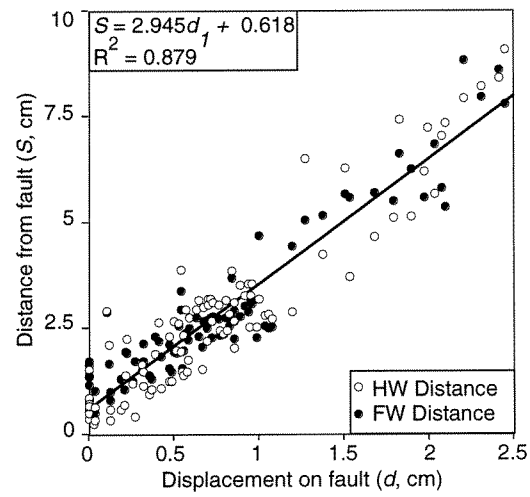
Figure 3.3. Linear relationship between local displacement and fault shield projection distance for master faults from this population.
