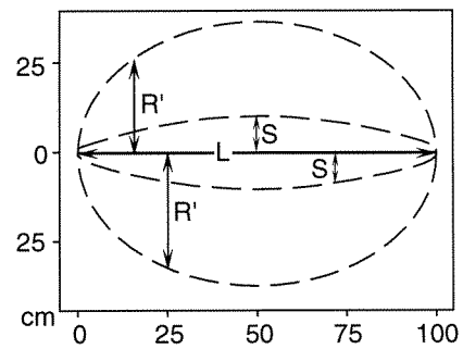
Figure 3.4. Map view of a simple model for the relationship between the deformation field and fault shield at the center of an isolated, blind, neo-formed normal fault. The extent of the fault shield will vary with rock properties and strain rate, and terminates where the stress locally exceeds the shear strength of the rock. L = 100 cm, d_{\max} = 3 cm, axial ratio = 2 (Gupta and Scholz, 1996).
