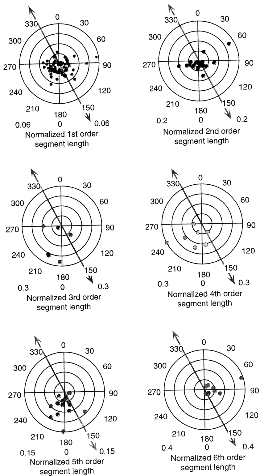
Figure 1.7b: Flow vector and structural data for Domain 15. See text for discussion.
