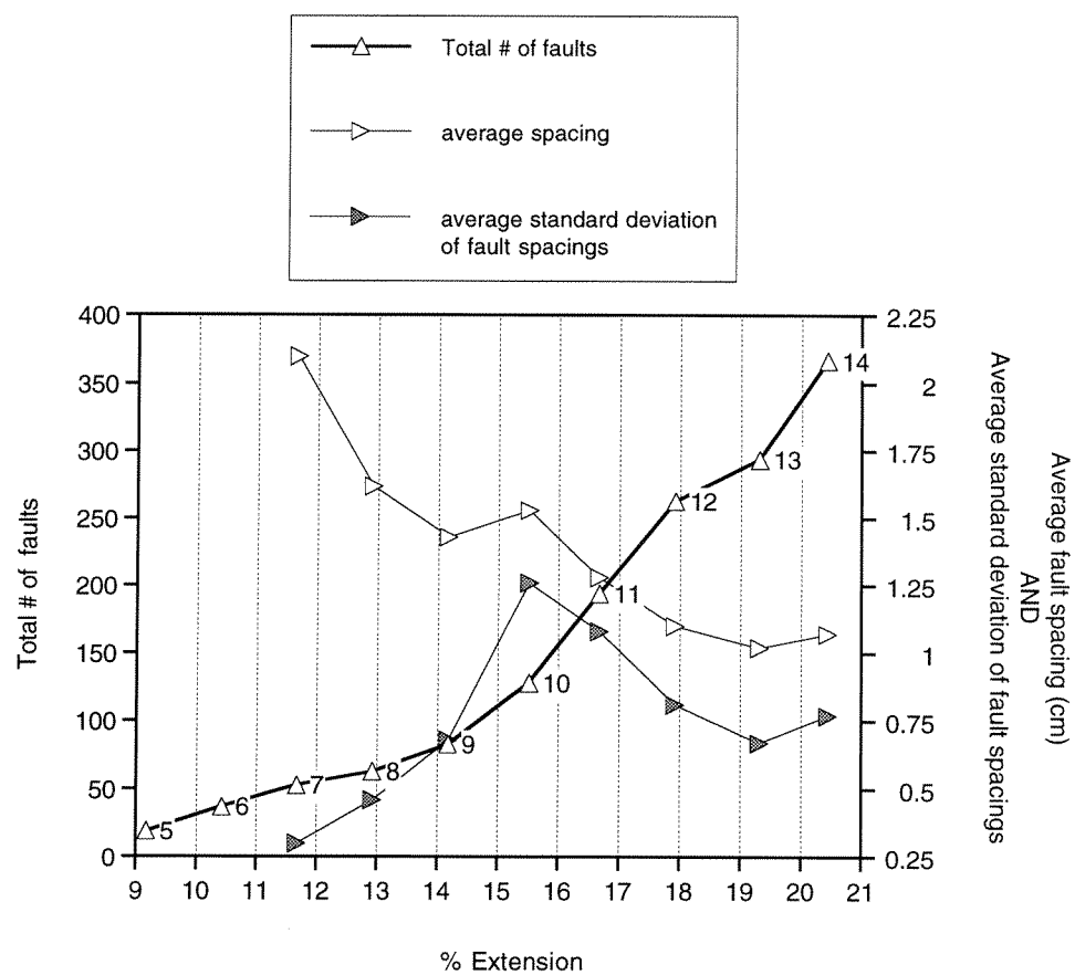
Figure 4.16: Total number of faults and fault spacing data through time.
