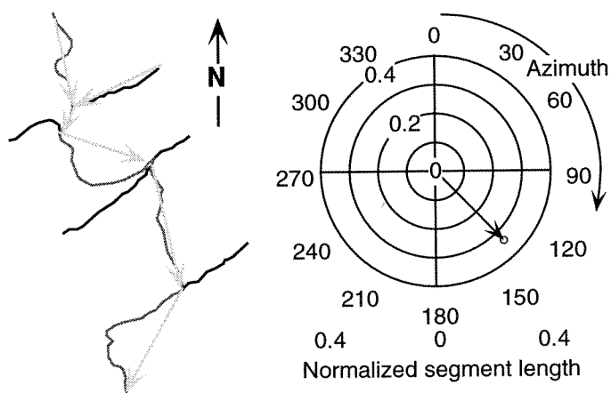
Figure 1.3: Method for determining channel segment flow vectors. Channels are broken down to confluence-confluence segments. Length components are normalized to the sum of the lengths for a given order by domain, and the normalized flow vectors are plotted on a polar diagram. The example point shown represents a channel segment with a normalized length of \sim 0.35 and a flow azimuth of \sim 135^\circ .
