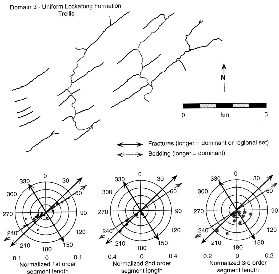
Figure 1.4: Streams, flow vector and structural data for Domain 3. See text for discussion.
