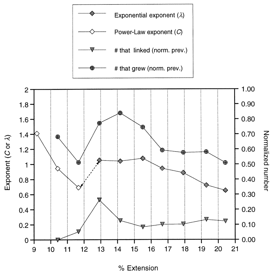
Figure 4.19: Cumulative frequency exponents, and normalized number of faults that linked and grew through time. See text for explanation of normalization.
