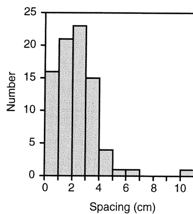
Figure 2.4: Histogram of spacings of macroscopic veins; notice undersampling at smaller spacing typical of outcrop-scale fracture studies.
