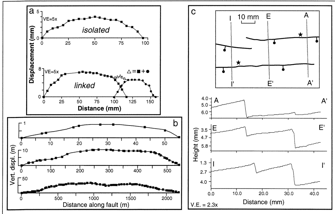
Figure 2.5: (a) Displacement versus distance plots for an isolated normal fault and a linked fault system from the Solite Quarry. Note that displacement gradients are higher at the tips of the linked faults, and that the summed displacement profile for the linked faults resembles that of an isolated structure, indicating that they are kinematically (soft) linked, although they are not breached (hard linked) in map view. Modified from Schlische et al. (1996). (b) Variations in scarp height for large normal faults from the Volcanic Tablelands, California. Note different horizontal and vertical scales; modified from Dawers et al. (1993). (c) Top: map of a bedding surface cut by three small normal faults from the Solite Quarry. Stars indicate locations of maximum displacement, shaded lines show locations of profiles across the offset bedding surface (bottom). Notice reverse drag immediately adjacent to the faults, as well as displacement transfer between the structures, maintaining strain continuity across the map area as one fault dies out.
