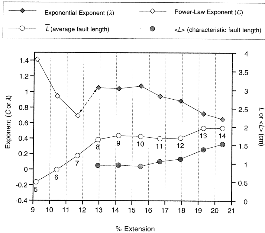
Figure 4.18: Cumulative frequency exponents, average lengths, and characteristic lengths through time. See text for full explanation.
