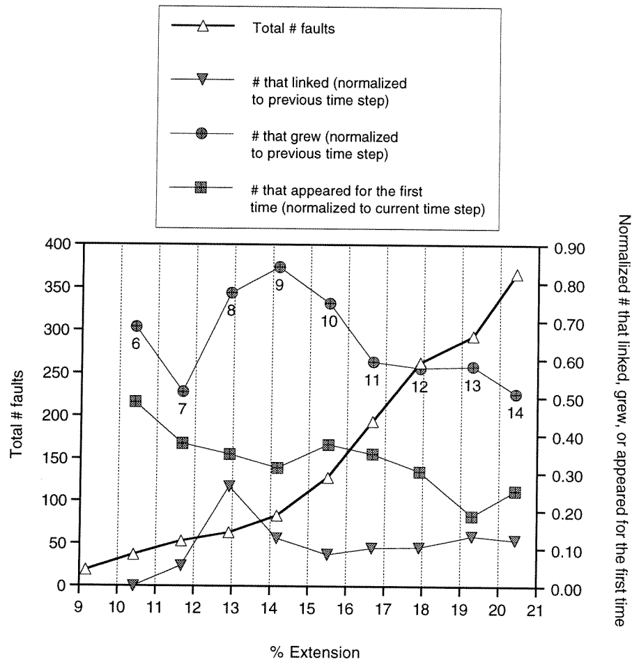
Figure 4.14: Total number of faults, and normalized number of faults that grew, linked, or appeared for the first time. See text for explanation of the normalization.
