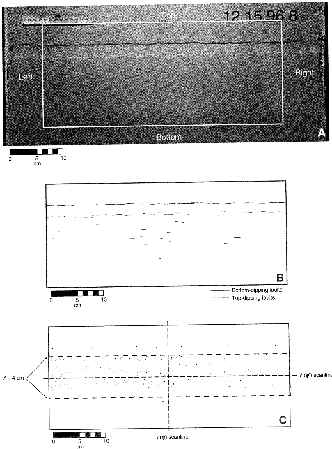
Figure 4.5: Time 8. A is the image of the model surface; the study area is outlined with the white box. B is the fault map derived from the image in A, C is the centroid map derived from B.
