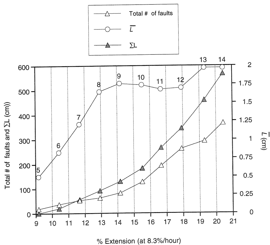
Figure 4.12: Number of faults, average length, and summed length through time (a constant strain rate of 1 cm/hr makes strain a proxy for time). Numbers above symbol are the time step.
