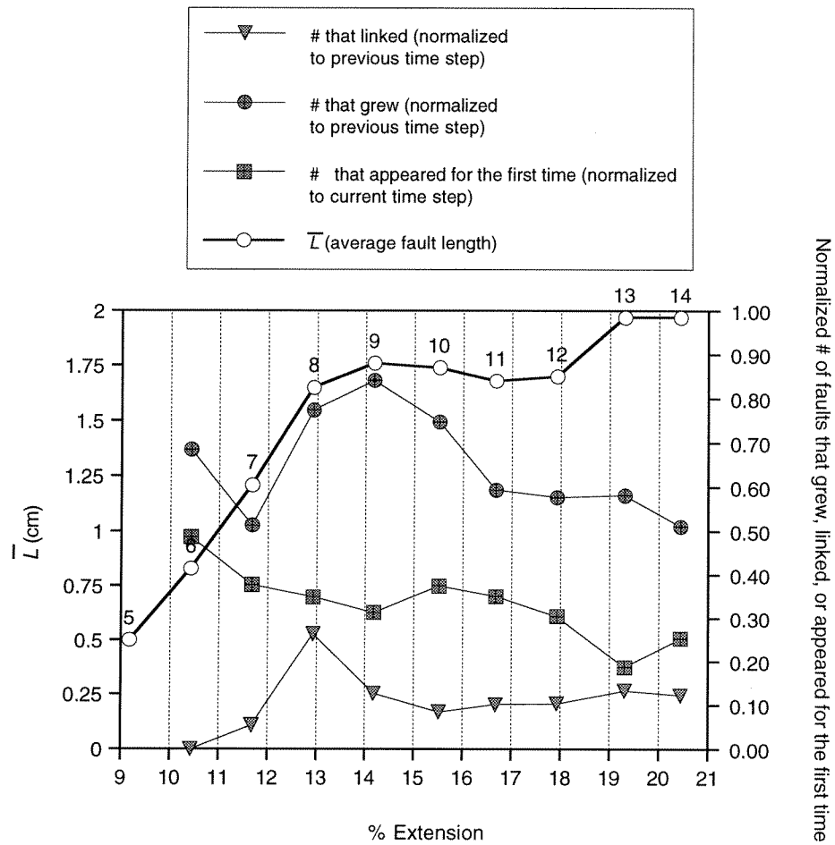
Figure 4.15: Average fault length and normalized numbers of faults through time.
