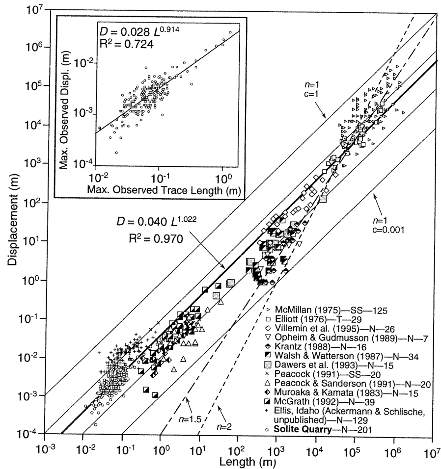
Figure 2.6: Log-log plot of displacement versus length for various published fault populations. Abbreviations are: N, normal faults; T, thrust faults; and SS, strike-slip faults. A family of linear curves ( n=1 ) with various c -values bound the data; the best-fit curve for all the data is shown as the heavy solid line. Also shown for reference are curves for n=1.5 and n=2 . Inset: Log-log plot of displacement versus length for only the small faults from the Solite Quarry, n \approx 1 .
