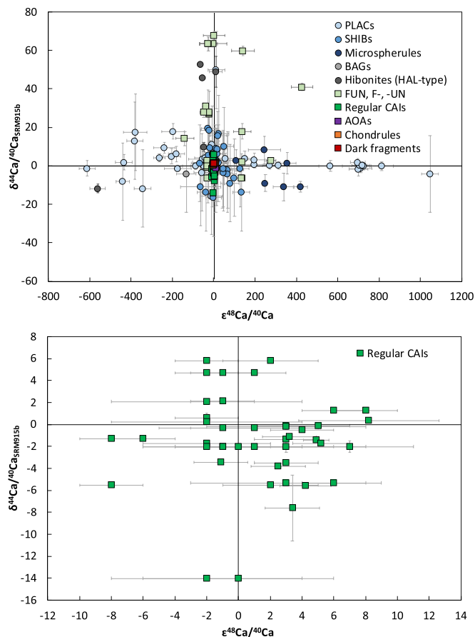
Fig. 3. Non-mass-dependent ( \epsilon^{48}\text{Ca}/^{44}\text{Ca} ) vs. mass-dependent ( \delta^{44}\text{Ca}/^{40}\text{Ca} ) isotopic compositions obtained from the same meteorite component. Error bars are those reported in the original publications. Mass-dependent data reported relative to SRM915a. The area around the origin in (a) is shown in (b) and displays regular CAIs only. The reader is referred to the web version of this article for the color version of this figure.
