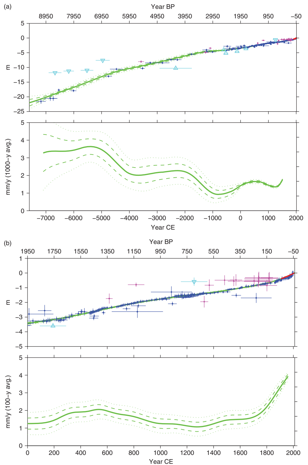
Figure 2. (a) Relative sea-level change over the past 10,000 years in New Jersey using dataset compiled by Horton et al. [2013] and Kemp et al. [2013] for basal (blue) and intercalated (magenta) dates and smoothed Atlantic City tide-gauge data (red); cyan = limiting dates with upward for marine limiting and downward for freshwater limiting, all with 2\sigma error bars. Smoothed line (green) along with 1\sigma (thick dashed line) and 2\sigma (thin dashed line) errors are shown. Bottom plot shows 1000 year average rates of change, plotted at the central year of each 1000 year interval. (b) Enlargement of the Common Era; smoothed line (red) along with 1\sigma (thick dashed line) and 2\sigma (thin dashed line) errors are shown. Bottom plot shows 100 year average rate of change, plotted at the central year of each 1000 year interval. See (a) for description.
