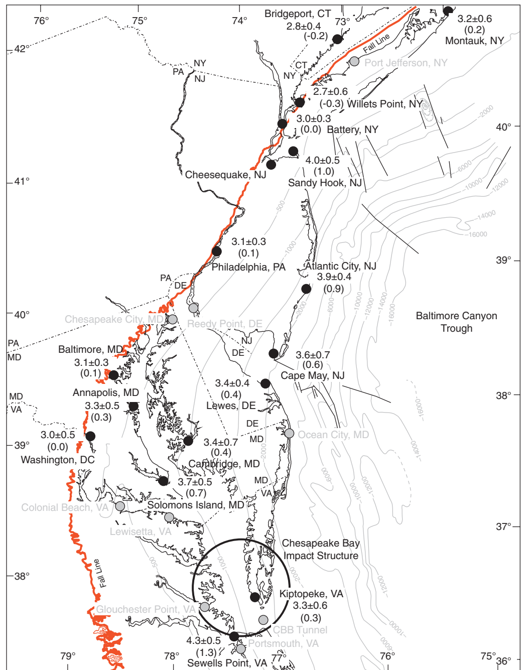
Figure 1. Relative sea-level rise and sea-level anomaly from tide-gauge data superimposed on geological map of Benson [1984]. Plotted are the linear trends from Kopp [2013] from 1900 and the subsidence anomaly derived by subtracting the trend at the Battery. Structural contours on the coastal plain and the Baltimore Canyon Trough are to basement in meters. Gray circles are tide gauges with insufficient length (<60 yr.). Red = Fall Line.
