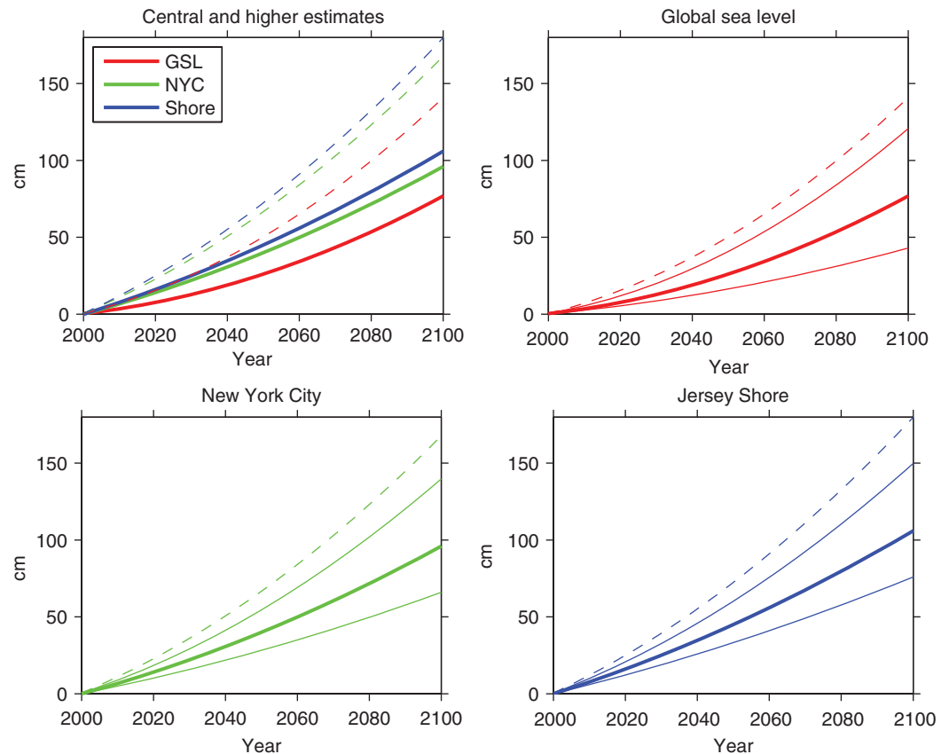
Figure 5. Projections of global sea-level (GSL) rise, relative sea-level rise at New York City, and relative sea-level rise on the Jersey shore. In the upper left plot, central (heavy solid) and higher (dashed) scenarios are shown for GSL (red), New York City (green), and the Jersey shore (blue). In the other three plots, low (solid) and high (upper solid) scenarios are also shown.
