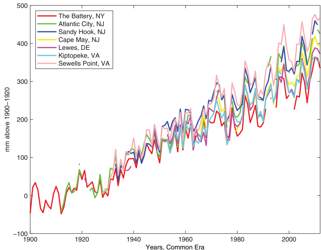
Figure 4. Comparison of tide gauges along the coast with the Battery. The tide-gauge records are referenced to a synthetic 1900–1920 datum, inferred based on the Gaussian process sea-level model of Kopp [2013].
