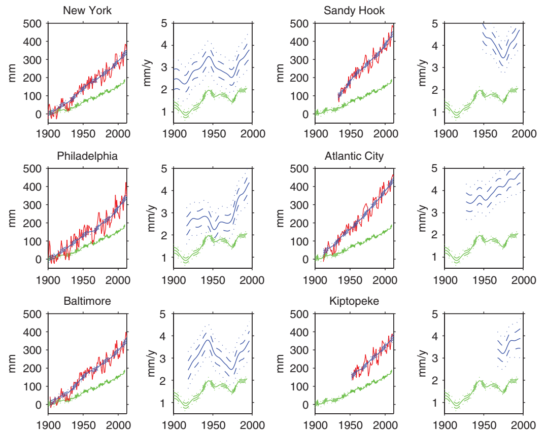
Figure 3. Examples of tide-gauge analyses for sites along the Fall Line (left columns) and in the coastal plain (right columns) [Kopp, 2013]. In the first panel for each site are the data (red), the modeled underlying sea level with red-noise-type variability removed (blue, see text for analysis procedure), and the average global sea level (GSL) derived from tide-gauge records [green, Church and White, 2011]. In the second panel are the 31 year average rates of change with 1\sigma (thick dashed lined) and 2\sigma (thin dashed line) uncertainties.
