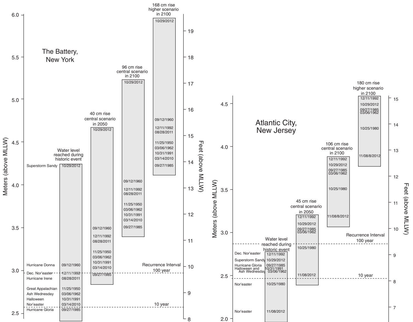
Figure 6. (a) Effects of sea-level rise on storm surge for the Battery assuming relative rises of 40 cm (2050 Common Era [CE]) and 96 cm (2100 CE) (our central scenario) for the first three columns and 168 cm (higher scenario) for 2100 CE for the fourth column. The Advisory Base Flood Elevation for this location is 4.6 m (15 ft mean lower low water, MLLW; 12 ft NAVD88; http://www.region2coastal.com/sandy/table ). Adapted after Psuty [1986]. (b) Effects of sea-level rise on storm surge for Atlantic City assuming relative rises of 45 cm (2050 CE) and 106 cm (2100 CE) (our central scenario) for the first three columns and 180 cm (higher scenario) for 2100 CE for the fourth column. The Advisory Base Flood Elevation for this location is 5.1 m (16.6 ft MLLW; 14 ft NAVD88; http://www.region2coastal.com/sandy/table ). Adapted after Psuty [1986].
