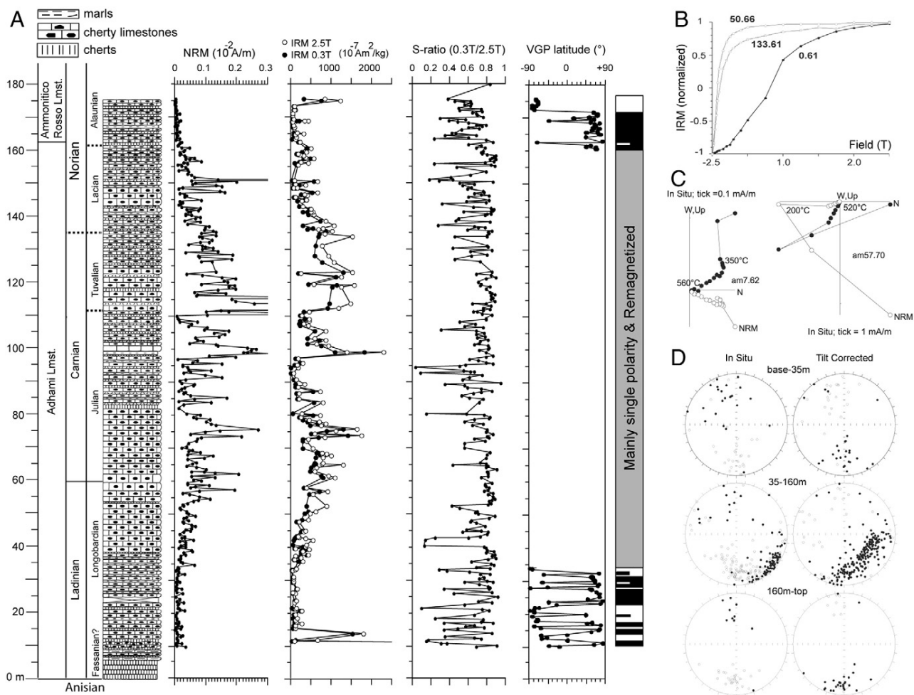
Fig. 4. Paleomagnetic data of the Aghia Marina section: (A) from left to the right: age and lithology, natural remanent magnetization (NRM), isothermal remanent magnetizations (IRM) at 0.3 T and 2.5 T (C), S-ratio (0.3 T/2.5 T), virtual geomagnetic pole (VGP) latitudes and magnetic polarity stratigraphy (black is normal, white is reverse, gray is unknown). (B) Isothermal remanent magnetization acquisition curves. (C) Vector end-point demagnetization diagrams (closed symbols are projections onto the horizontal plane and open symbols onto the vertical plane in geographic [in situ] coordinates). (D) Equal-area projections of magnetic component directions before (in situ) and after bedding tilt correction (closed symbols are projections onto the lower hemisphere and open symbols onto the upper hemisphere).
