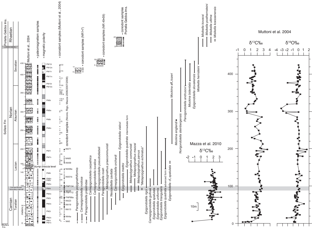
Fig. 5. Pizzo Mondello section. From left to the right: age, lithology, magnetostratigraphy, conodont biostratigraphy, and bulk-rock \delta^{13}C and \delta^{18}O data. See also Mazza et al. (2012a) for a detailed biostratigraphic record.
